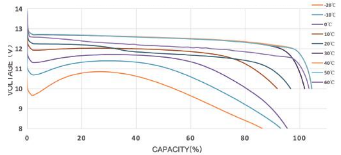
DIFFERENT TEMPERATURE DISCHARGE CURVE (0.5C)
