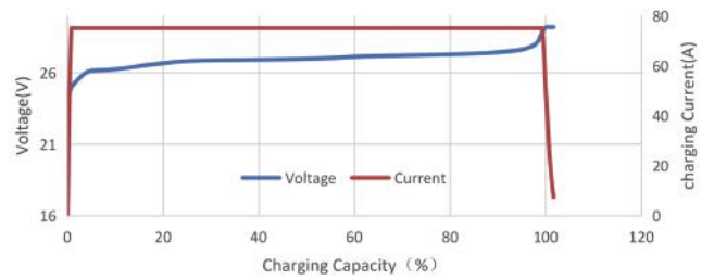
STATE OF CHARGE CURVE (0.5C, 25°C)
