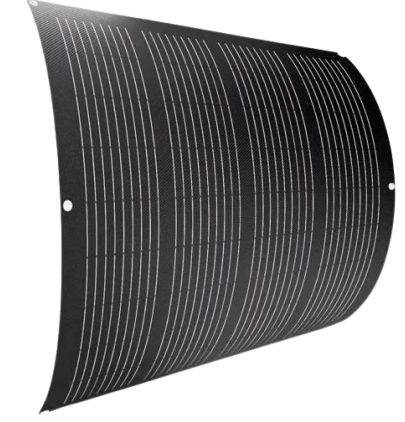
Flexible Panel 4 x200W, 3.3KG 1140*915*18mm
